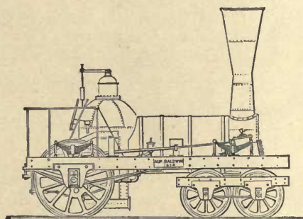
Fig. 3.—BALDWIN ENGINE, 1834.
