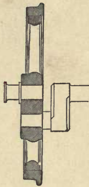
Fig. 2.—HALF-CRANK.
